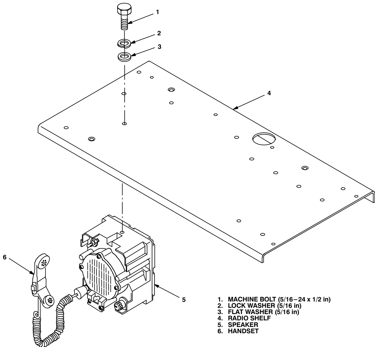
Figure 5-13. Speaker Installation
